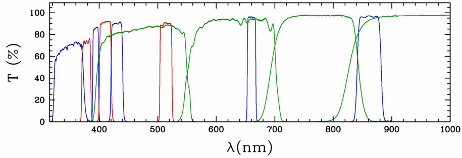
Figure 1: The measured transmission curves of the J-PLUS filters mounted on T80Cam
