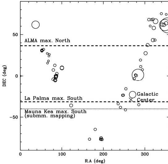
Figure 1. The distribution of known Class 0 objects on the sky, with approximated maximum ranges for ALMA (towards the North) and telescopes in La Palma and Hawaii (towards the South). Circles areas are proportional to the source distance. Lines correspond to air masses equal 2.0. (Courtesy of D. Barrado Navascués, Centro de Astrobiología).
