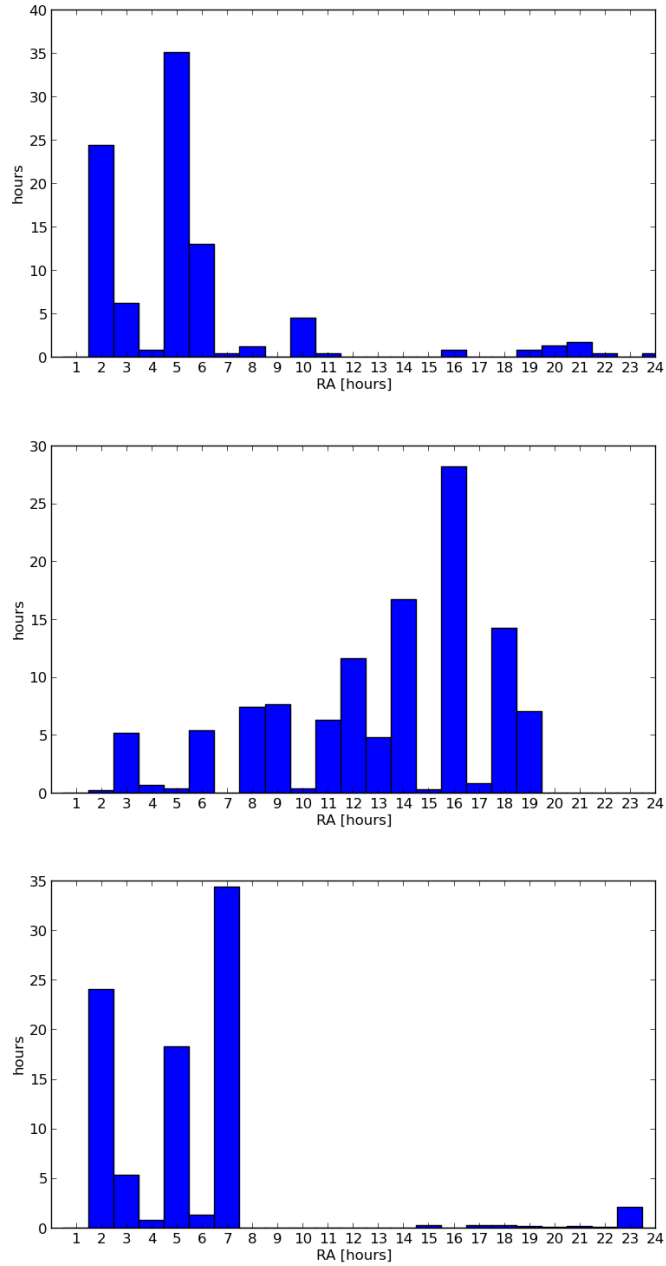
Figure 3: The time requested distributed in the different intervals of right ascension for periods, from top to bottom, 2016B, 2017A, and 2017B. Note that, for obvious reasons, ToO programs are not included in this plot.
