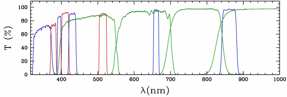
Figure 1: The measured transmission curves of the J-PLUS filters mounted on T80Cam
