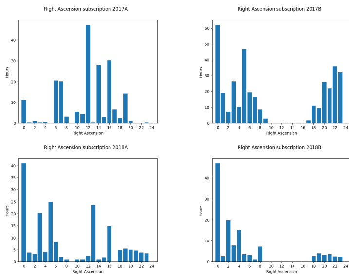
Figure 3: The time requested distributed in the different intervals of right ascension from 2017A to 2018B for granted proposals.
